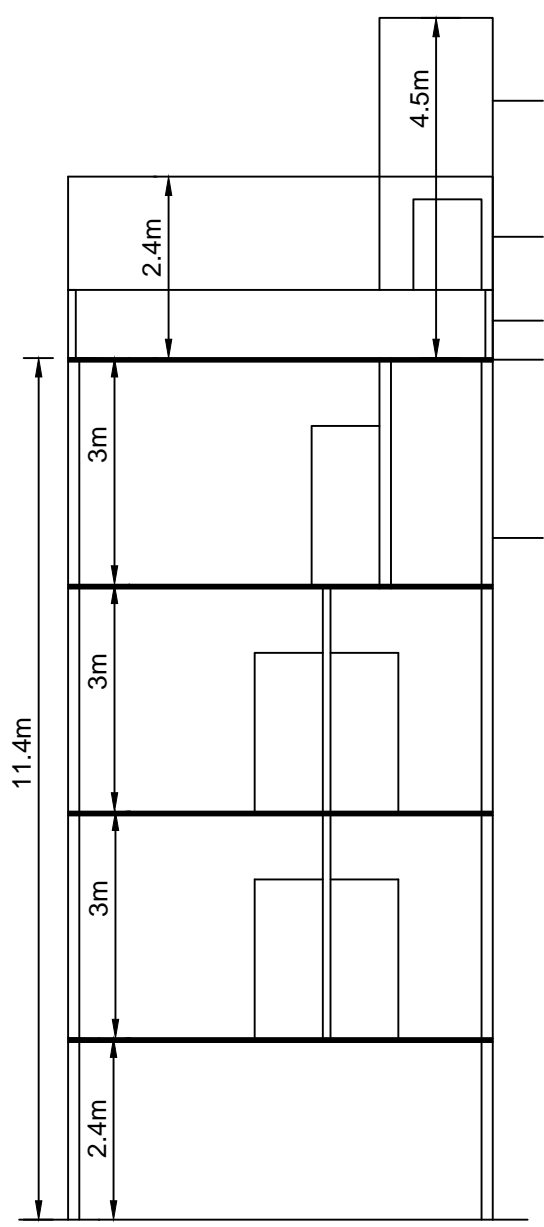
SECTION @ X-X
